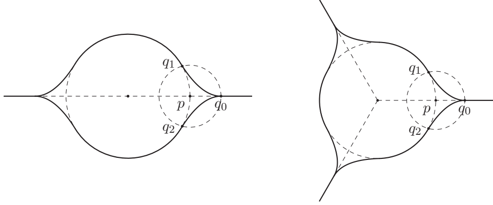
FIGURE 3. The set O_R constructed in Definition 3.4, depending whether \mathcal{E}_0 has two infinite regions (left) or three infinite regions (right).
